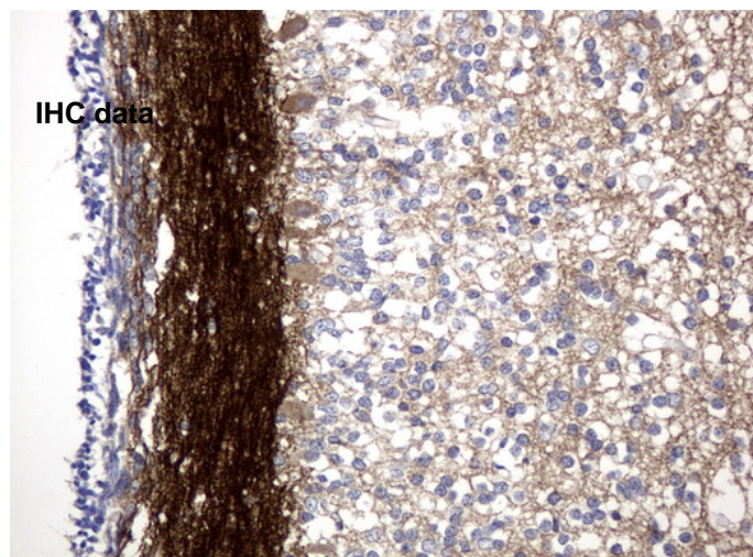
Immunohistochemical staining of paraffin-embedded Human embryonic cerebellum using anti-L1CAM mouse monoclonal antibody. (UM500043)
